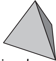
triangular based pyramid
