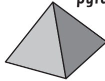
square based pyramid
